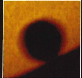
Black-Drop Effect
