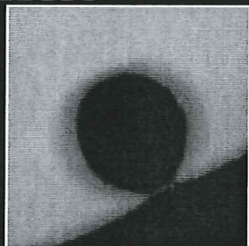
Black-Drop Effect
