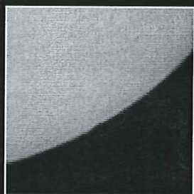
Egress Sequence
