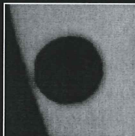
Transit Maximum
