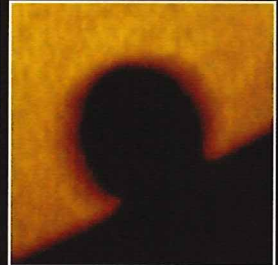
Transit Maximum
