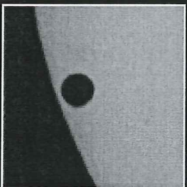
Ingress Sequence
