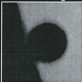
Black-Drop Effect
