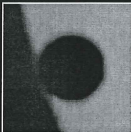
Black-Drop Effect
