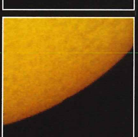
Egress Sequence
